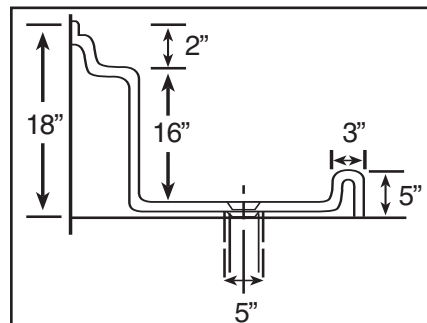
Single Threshold with seat
